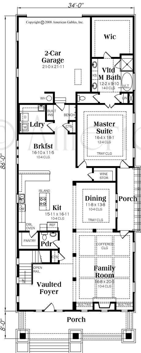
1ST FLOOR
